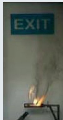
Smoke formation of PVC, PS, SAN, PC, PETG, shown here by the example of PC (rated B1, flame-resistant, to DIN 4102)
